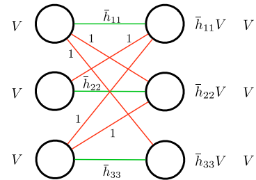
Fig. 19: Normalized channel of structure K
