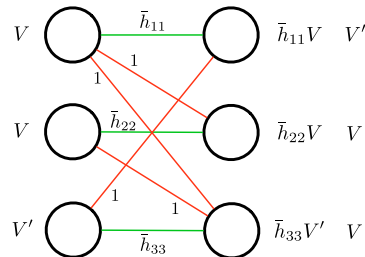
Fig. 16: Normalized channel of structure H
