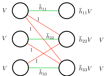
Fig. 15: Normalized channel of structure G
