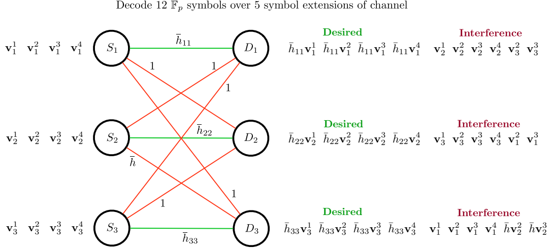
Fig. 10: 3-user Interference channel over \mathbb{F}_{p^2}
