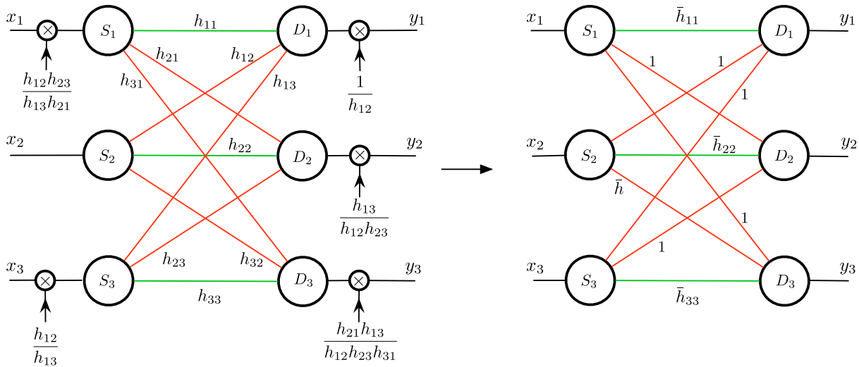
Fig. 7: Normalization in 3-user Interference Channel
