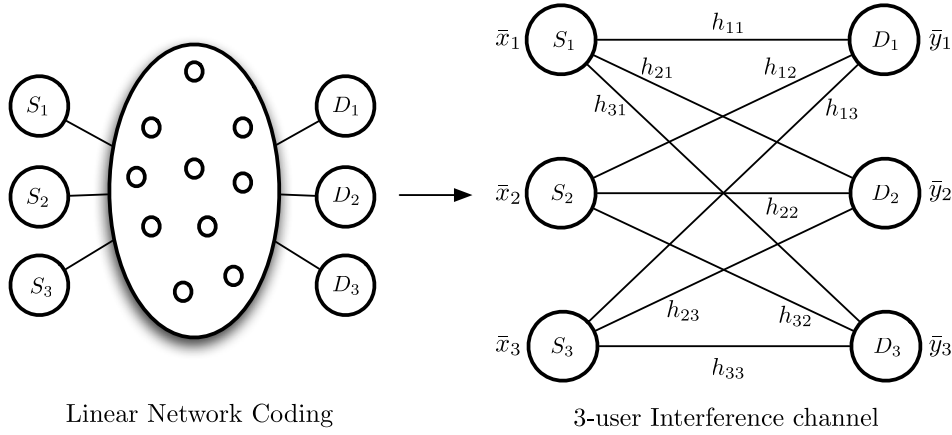
Fig. 6: Wired network modeled as 3-user interference channel
