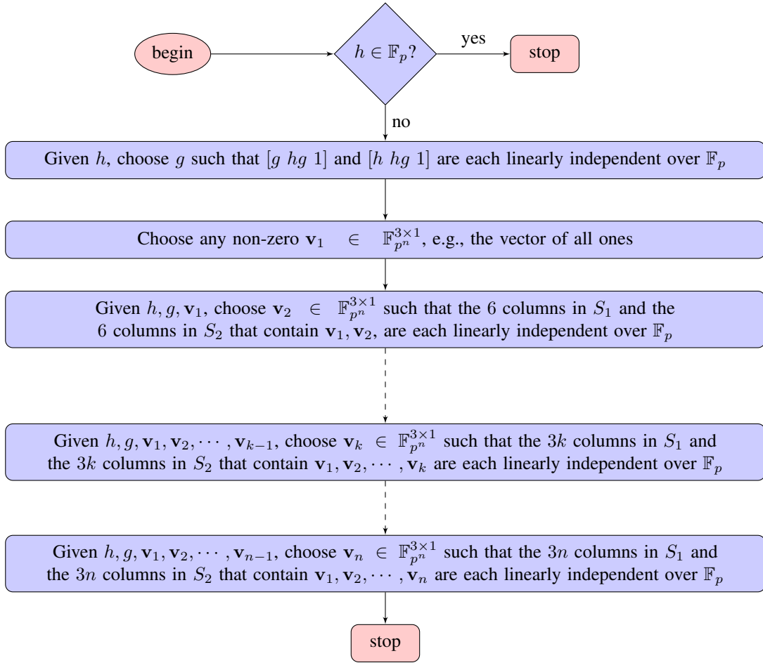
Fig. 5: Algorithm for the construction of precoding vectors.
