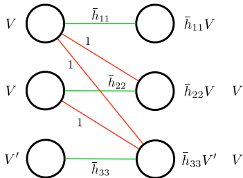
Fig. 13: Normalized channel of structure D
