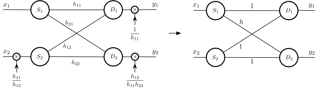
Fig. 2: Normalization in X channel
