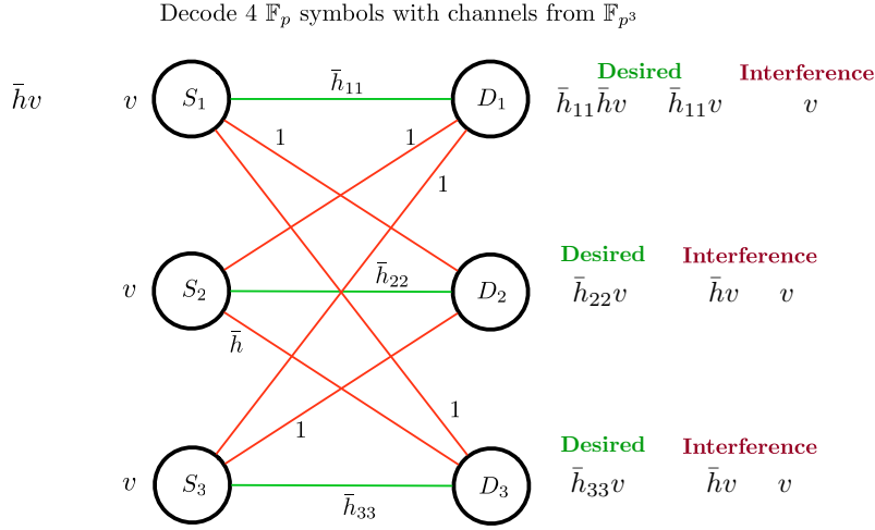
Fig. 8: 3-user Interference channel over \mathbb{F}_{p^3}
