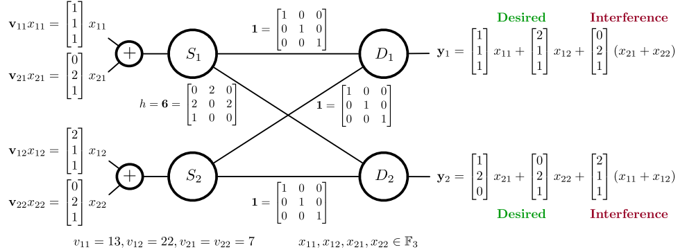
Fig. 4: The same example and solution as Fig. 3, illustrated in vector notation.
